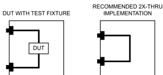
Figure 6—2X-Thru implementation
