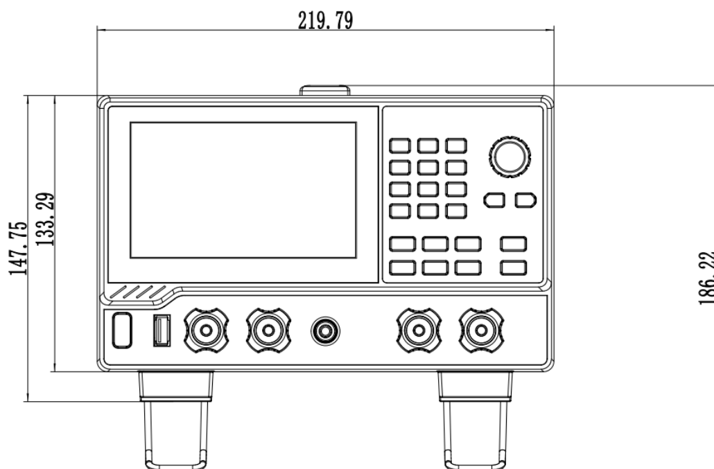
正视图 (SPB3100X, SPB3200X)
