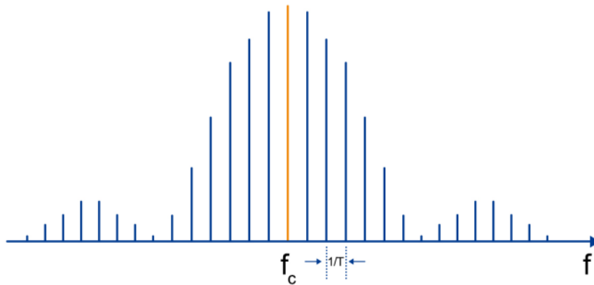
Figure 2-2 spectrum of radio frequency pulse signal
