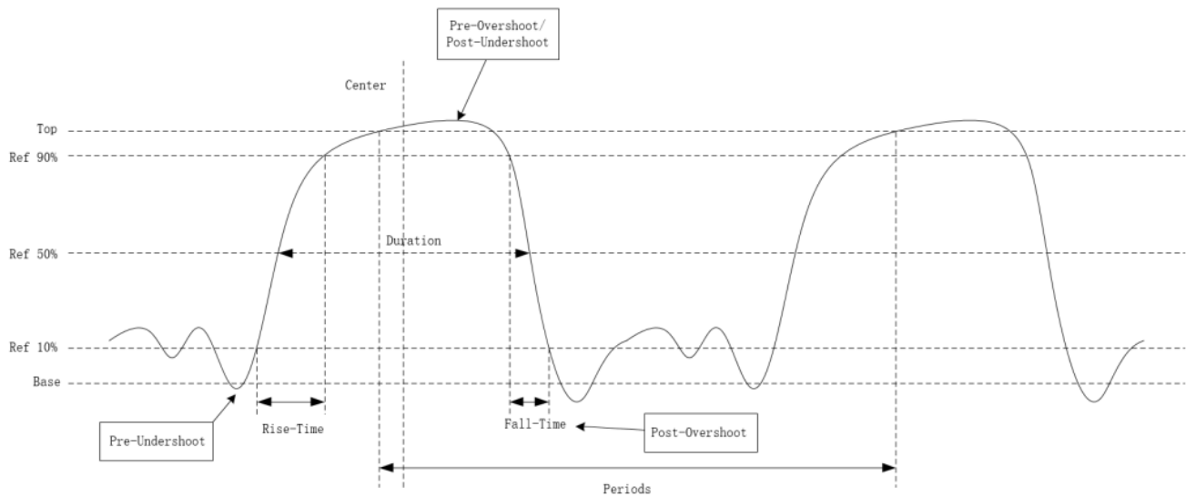
Figure 3-2 Pulse Signal Schematic
