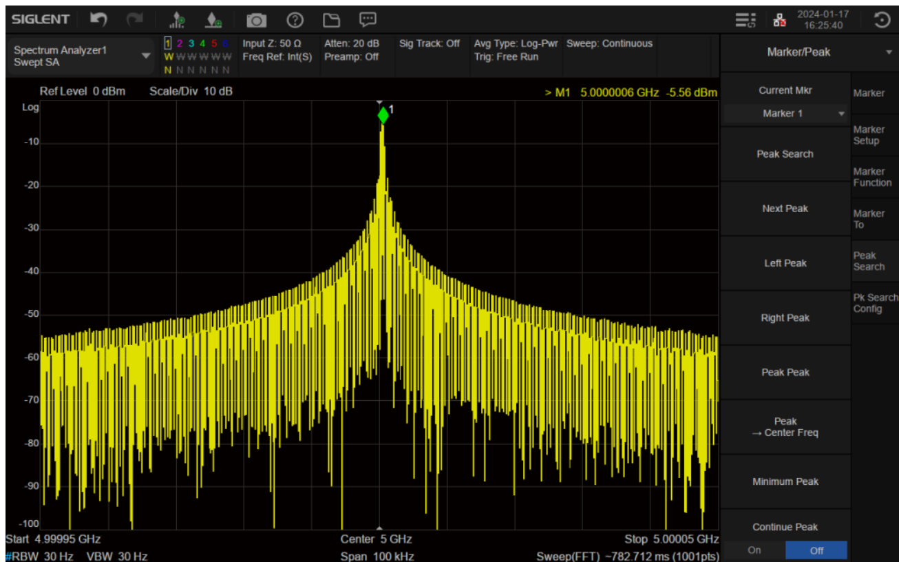
Figure 4-1 Spectrum of pulse modulation in SA mode
