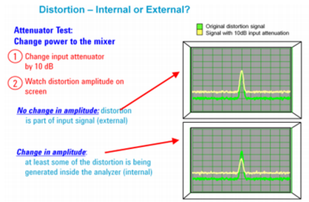
Figure 9: A technique to determine the source of distortion.
