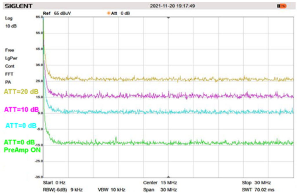
Figure 8: DANL versus internal attenuator / pre-amplifier settings. RF input terminated with 50 Ohm.
