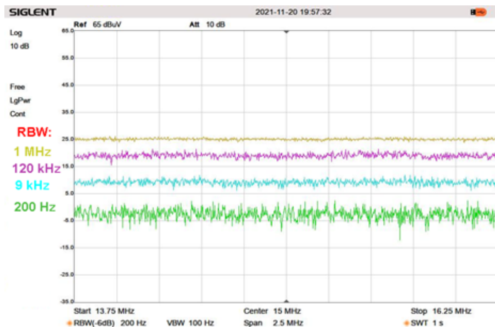
Figure 3: Spectrum analyzer DANL level versus resolution bandwidth.
