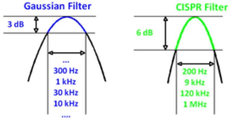
Figure 1: Gaussian and CISPR filter shapes.
