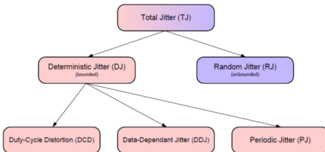
Figure 7: Jitter Decomposition
