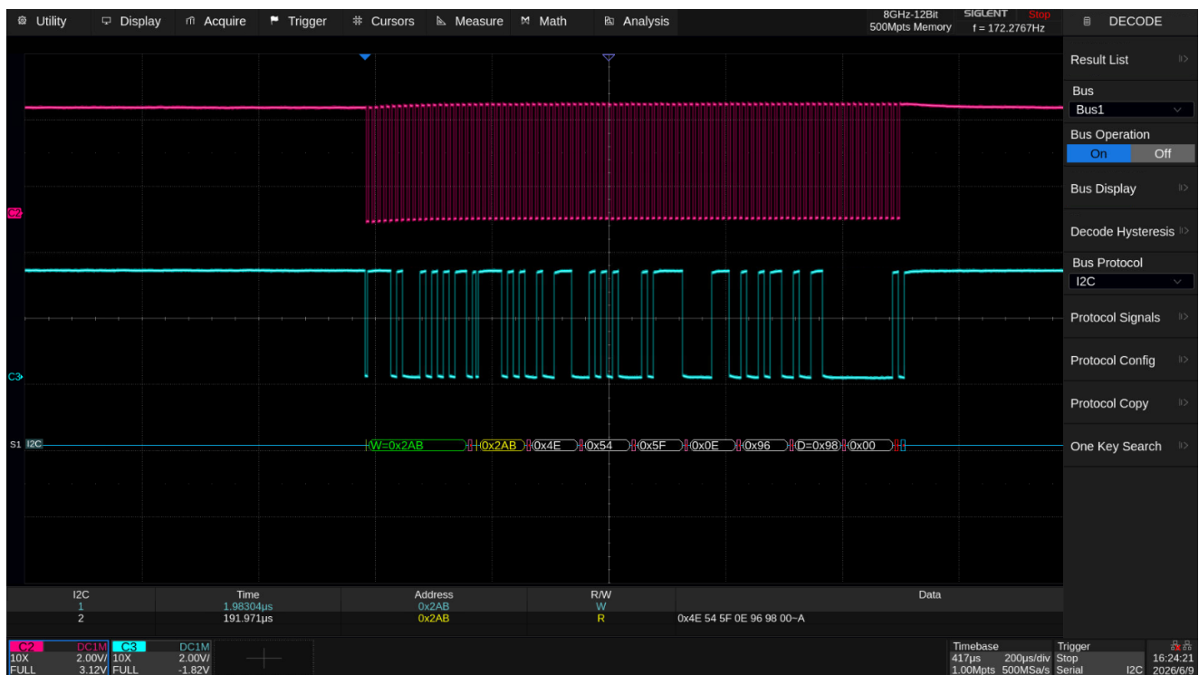
Figure 6: I2C Decode Results
